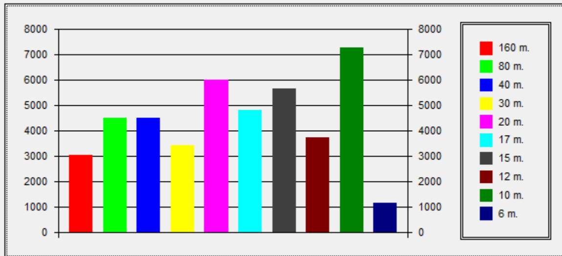
PT0S QSO Count per Band
